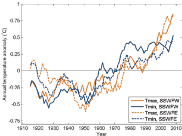
FIGURE 4.2.1: OBSERVED ANNUAL MEAN TEMPERATURE ANOMALIES ( ^{\circ}\text{C} ) FOR 1910–2013 COMPARED TO THE BASELINE 1986–2005 FOR (A) SSWFW AND (B) SSWFE. CLUSTER AVERAGE DATA ARE FROM ACORN-SAT AND GLOBAL DATA ARE FROM HADCRUT3V (BROHAN ET AL. , 2006).
