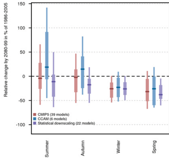
FIGURE 4.4.5: PROJECTED CHANGE IN SSWF SEASONAL RAINFALL FOR 2090 USING CMIP5 GCMS AND TWO DOWNSCALING METHODS (CCAM AND SDM). RAINFALL ANOMALIES ARE GIVEN IN PERCENT WITH RESPECT TO 1986–2005 UNDER RCP8.5. BAR PLOTS ARE EXPLAINED IN BOX 4.2.
