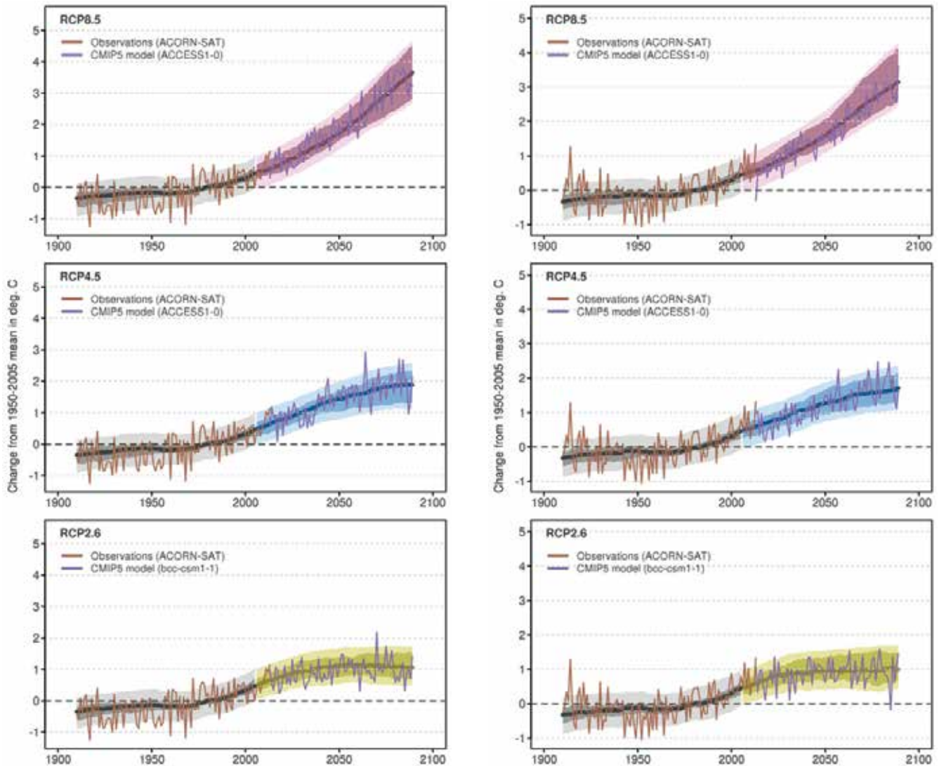
FIGURE 4.2.4: TIME SERIES FOR ANNUAL AVERAGE SURFACE AIR TEMPERATURE (°C) FOR 1910–2090, AS SIMULATED IN CMIP5 RELATIVE TO THE 1950–2005 MEAN. PANELS ON THE LEFT ARE SSWFW AND PANELS ON RIGHT SSWFE. THE CENTRAL LINE IS THE MEDIAN VALUE, AND THE SHADING IS THE 10TH AND 90TH PERCENTILE RANGE OF 20-YEAR MEANS (INNER) AND SINGLE YEAR VALUES (OUTER). THE GREY SHADING INDICATES THE PERIOD OF THE HISTORICAL SIMULATION, WHILE THREE FUTURE SCENARIOS ARE SHOWN WITH COLOUR-CODED SHADING: RCP8.5 (PURPLE), RCP4.5 (BLUE) AND RCP2.6 (GREEN). ACORN-SAT OBSERVATIONS AND PROJECTED VALUES FROM A TYPICAL MODEL ARE SHOWN. TIME SERIES PLOTS ARE EXPLAINED IN BOX 4.2.
